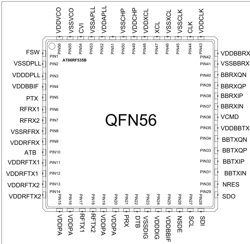
Figure 3. Pin Information
